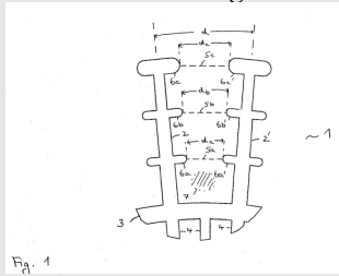
Heat exchanger
